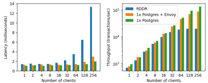
Fig. 5: Throughput and latency for 10,000 transactions per client.
